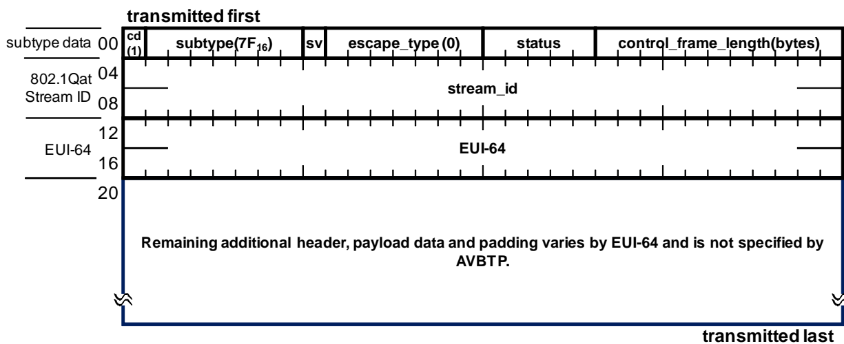
Figure 7.2—Proprietary/Experimental control escape subtype format
