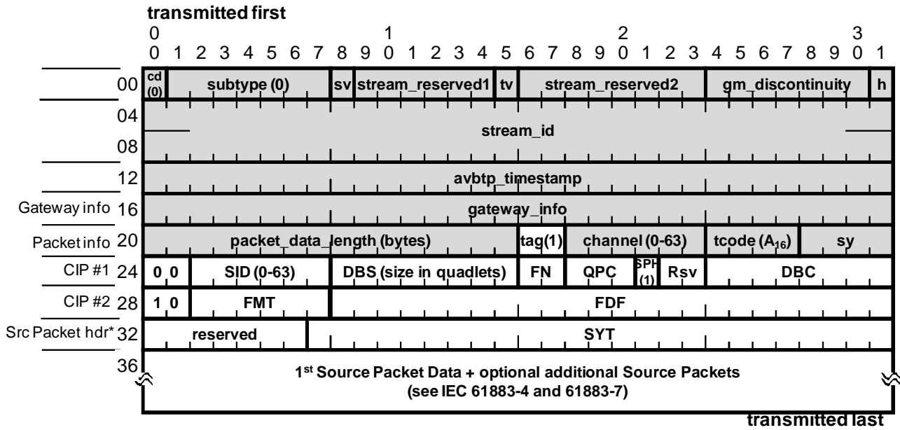
Figure 6.4—CIP header and data fields, tag=1, SPH = 1
