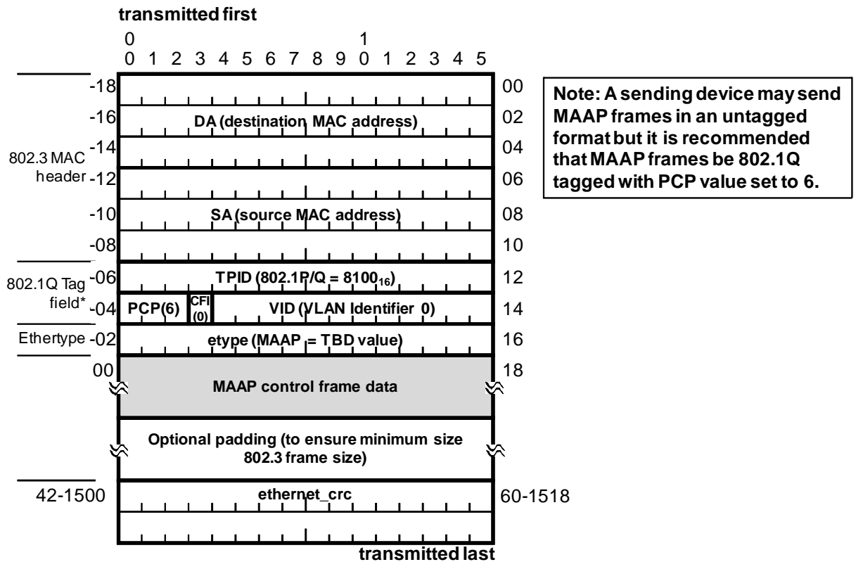
Figure C.1 – 802.3 MAAP frame format
