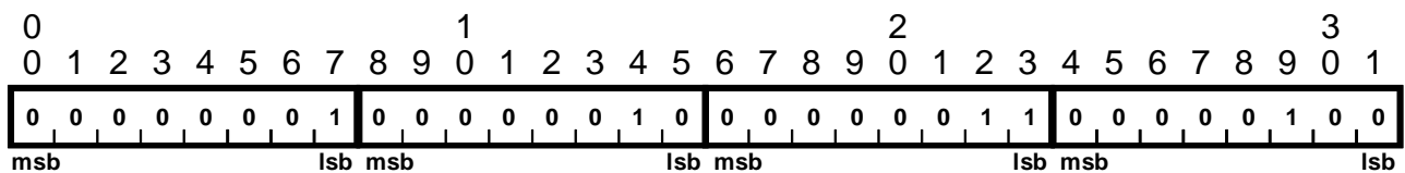
Figure 3.2 - Byte ordering within a quadlet
