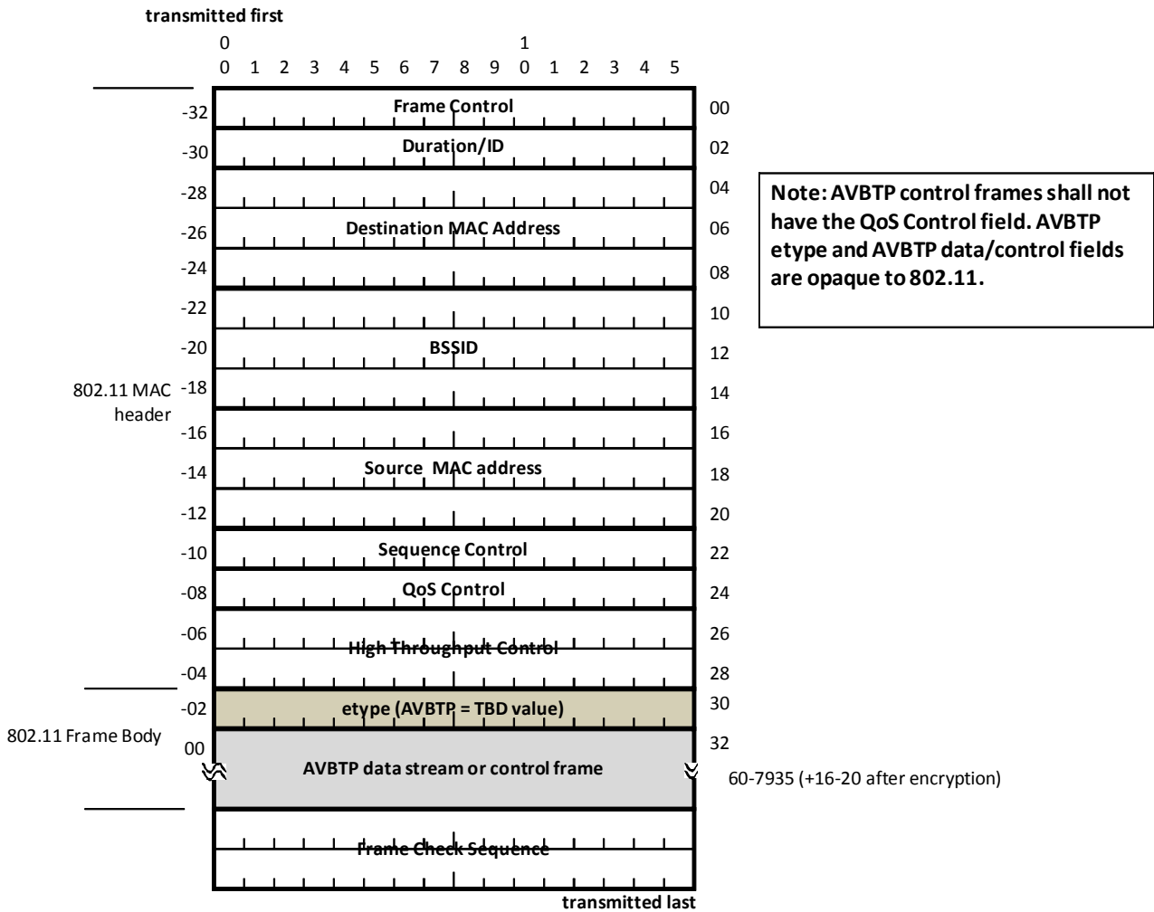
Figure 5.3 - AVBTP frame within an 802.11 frame
