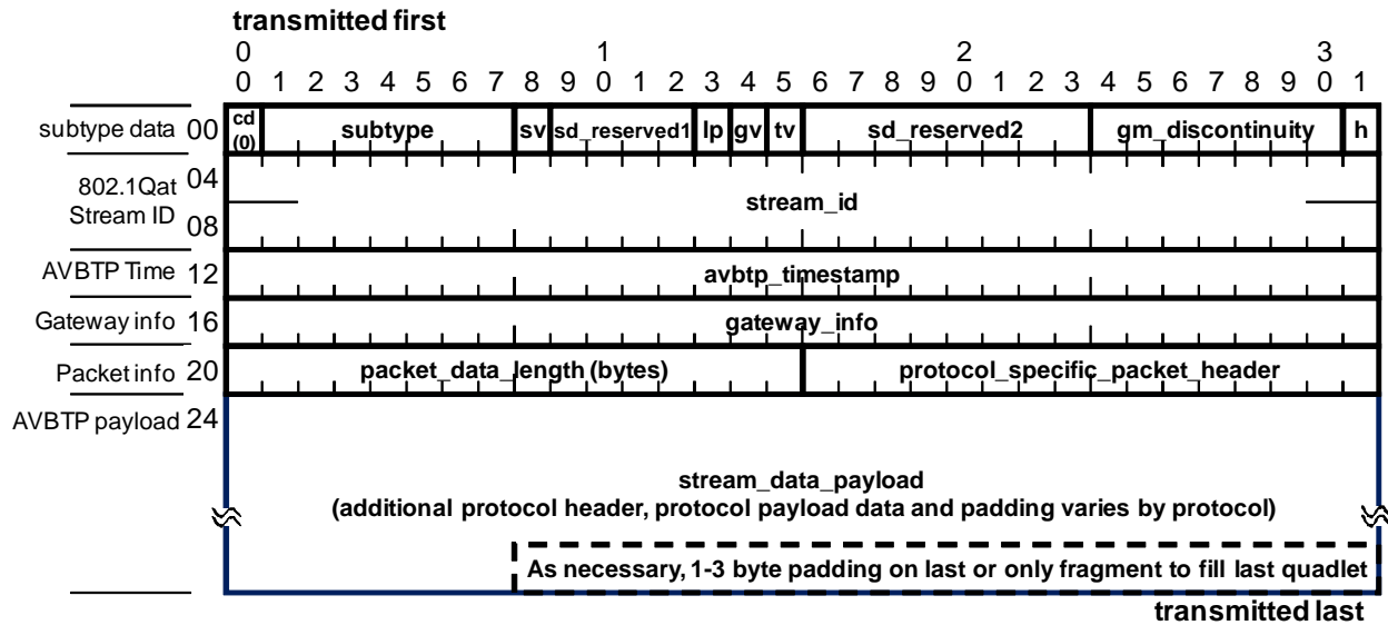
Figure 5.6 --AVBTP common stream data header format (cd field set to zero)
