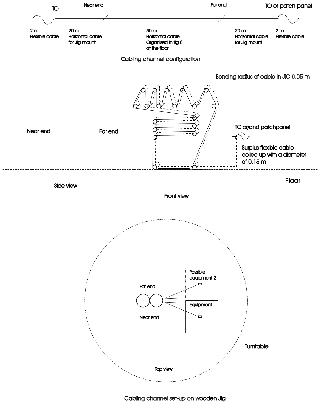
Fig. 1. Cabling set-up
