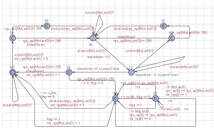
Figure 5-2 Registrar State Machine
