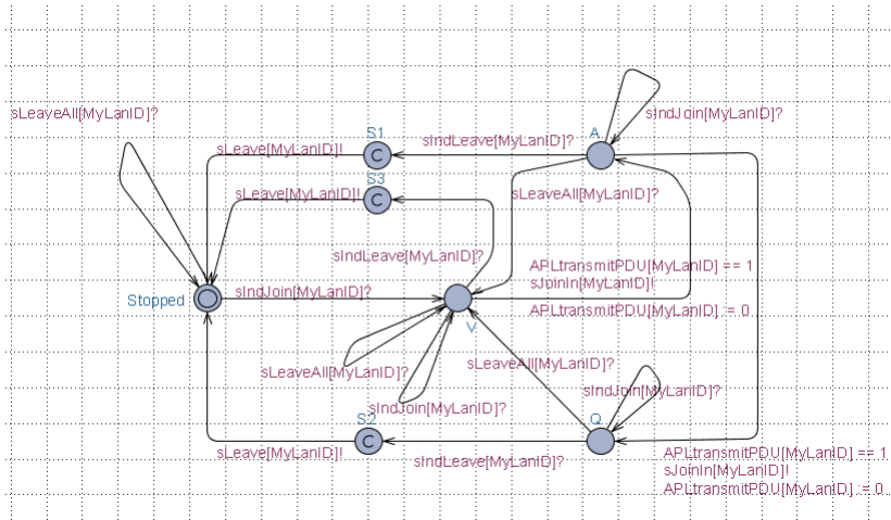
Figure 5-1 Applicant State Machine
