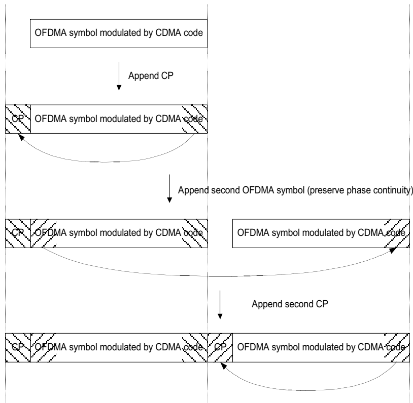
Figure 228 Initial-Ranging Transmission for OFDMA
