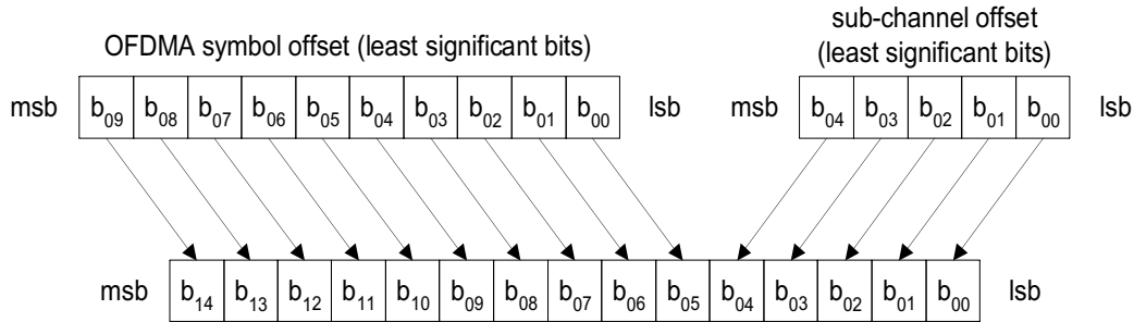
Figure 227 Creation of OFDMA Randomizer Initialization Vector
