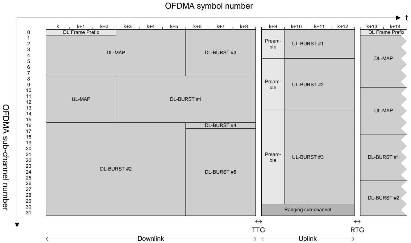
Figure 128ax—Time Plan - One TDD time frame
