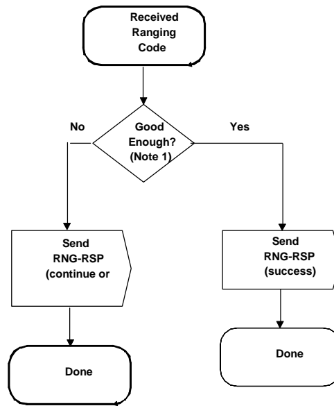
Figure 55b-Periodic ranging - Received Ranging Code - BS
