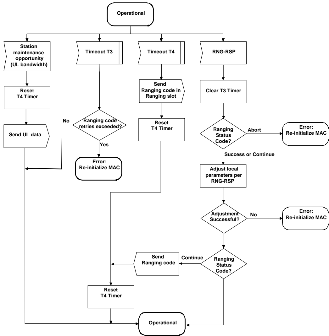
Figure 56-Periodic ranging - SS (CDMA ranging case)
