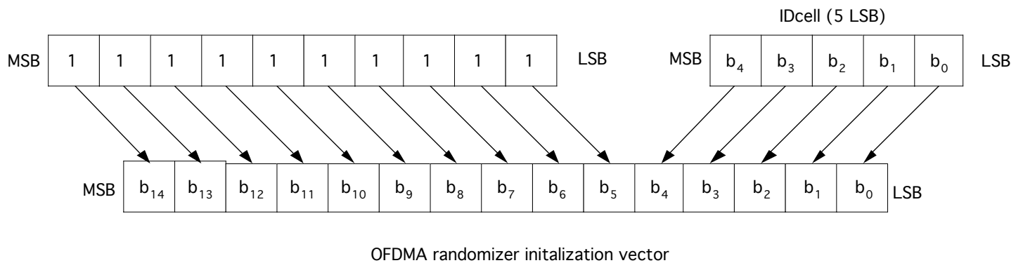
Figure 261—Initialization construction for the PRBS of the randomizer
