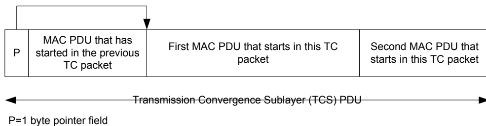
Figure 1. TCS PDU Format
