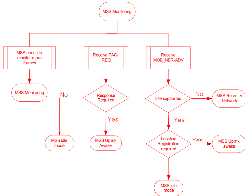
Figure xxx+2. - MSS Monitoring in Idle mode SDL Diagram
