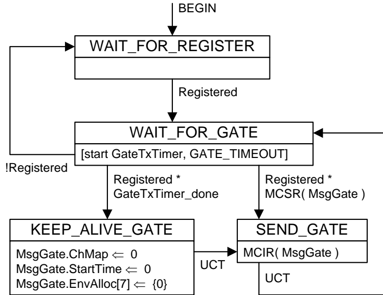
Figure 144-24 – Gate Generation state diagram
