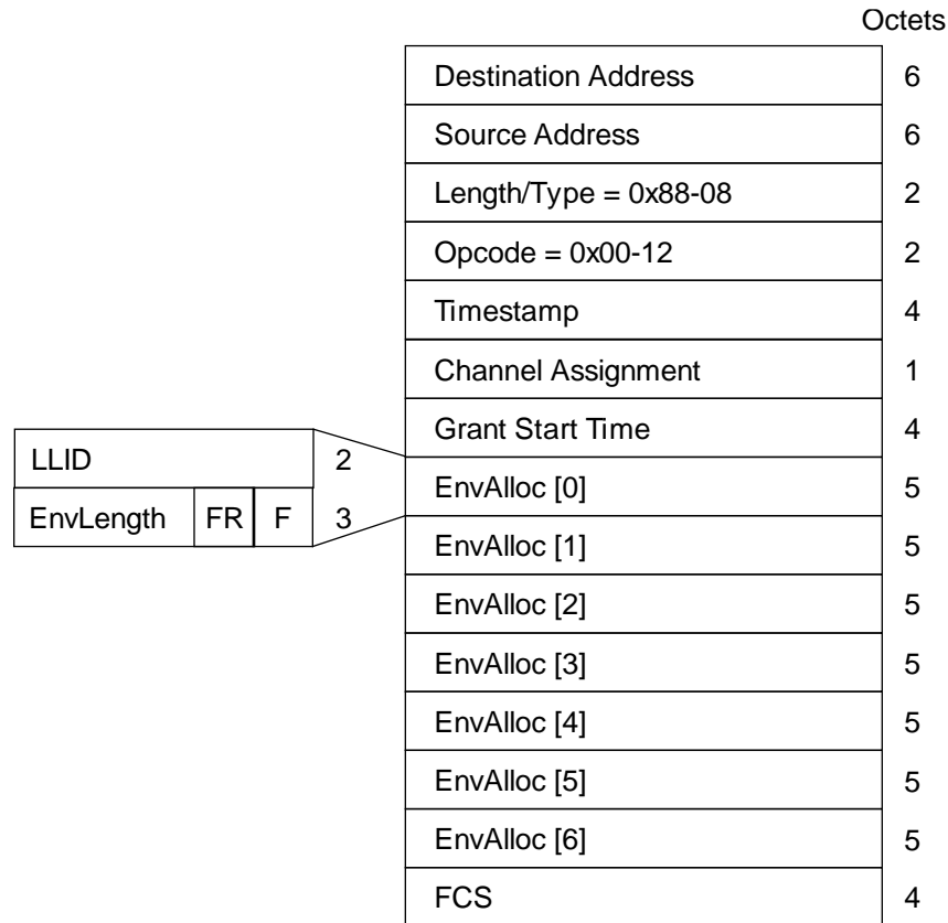
Figure 144-31—REPORT MPCPDU
