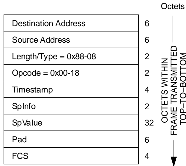
Figure 144–37—SYNC_PATTERN MPCPDU
