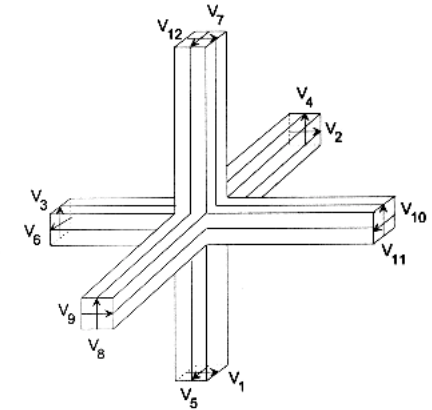
Figure 4: The Symmetrical Condensed Node
