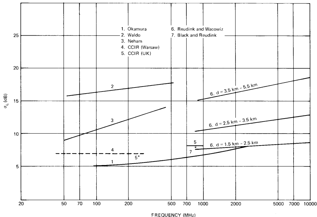
Figure 7— Standard Deviation of Location Variability \sigma_L , as a Function of Frequency in Urban Areas
