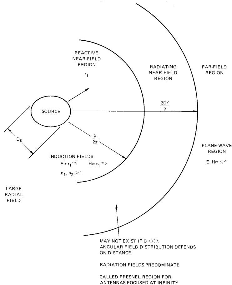
Figure 13— Source Regions
