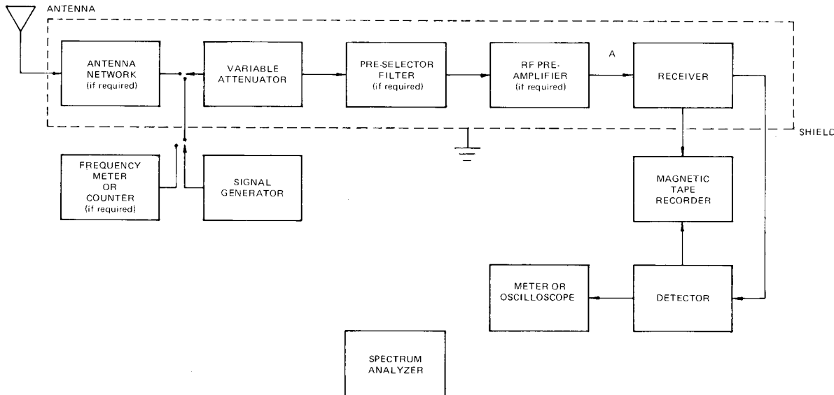
Figure 14— Measuring System
