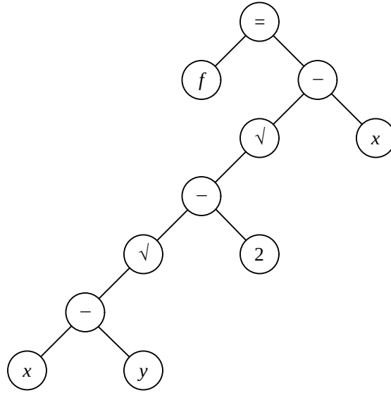
Figure 1: Syntax Tree
