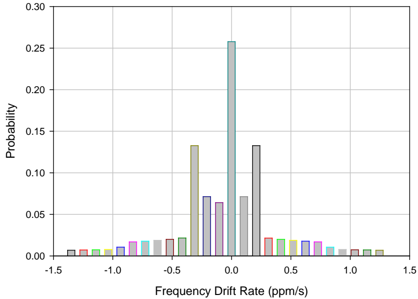
Probability Histogram for Frequency Drift Rate
