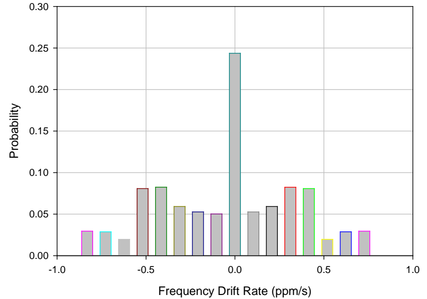
Probability Histogram for Frequency Drift Rate
