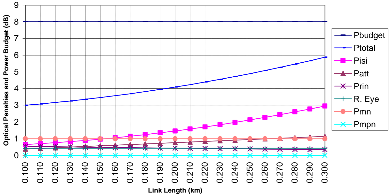
Graph 1 10Gbps Analysis for 2200 MHz-km 50 um Fiber at 850 nm
