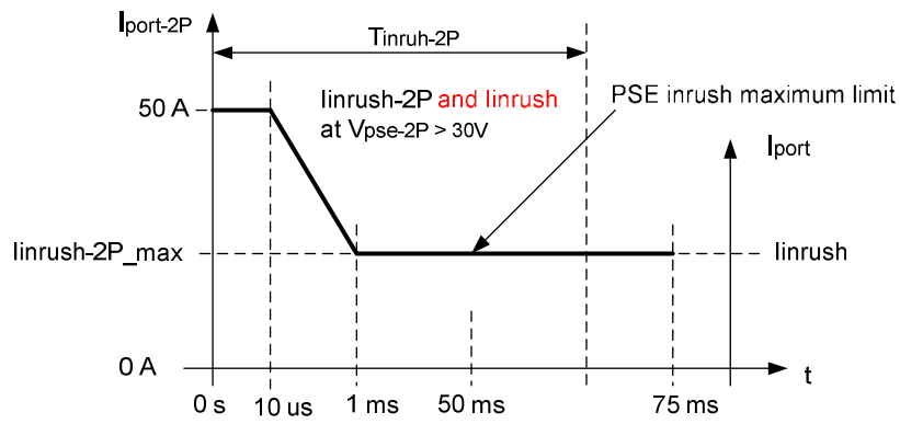
Figure 33-13 – I_{inrush-2P} and I_{inrush} current and timing limits, per pairset in POWER_UP
