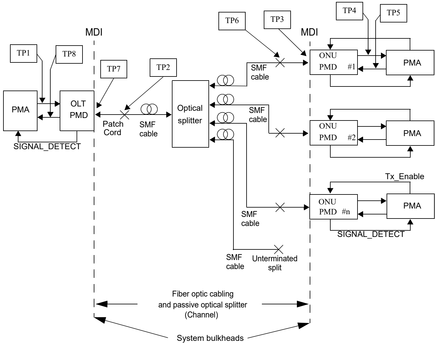
Figure 75-3—10GBASE-PR and 10/1GBASE-PRX block diagram
