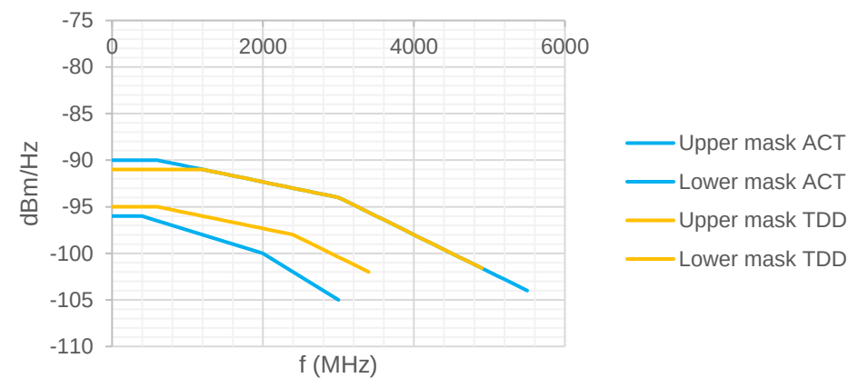
PSD masks, STP, Upstream
