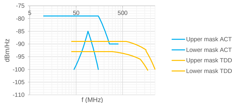
PSD masks, STP, Upstream
